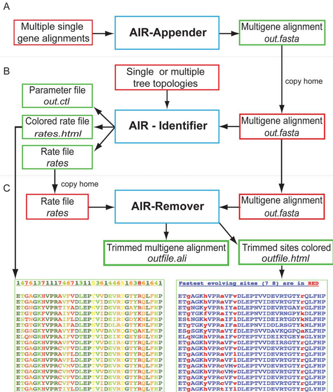
Figure 1 Overview of AIR-package. Overview of the functionalities and programs in the AIR-package installed on the Biportal: The colored boxes depict input files (red), output files (green), and the AIR programs (Blue). Texts in Italics depict the filename and respective extension of output files of AIR programs. A) AIR-Appender uses several single gene alignments for construction of a multigene alignment. B) AIR-Identifier uses the output file from AIR-Appender and file containing one or more phylogenetic trees for calculating site rates and rate categories. C. AIR-Remover deletes fast evolving sites according to settings defined by the user. The output files from each of the AIR programs can be used in subsequent analysis by copying the files from the work directory to project folder on the Biportal using the copy home function. Five main output files are produced by AIR. In which two are graphical html files with information about site rates and fast evolving sites ( rates.html ), and sites removed from the alignment ( outfile.html ). File 'rates.html' shows the rate categories as different colors (up to 8 categories), while 'outfile.html' shows the removed sites in red color (e.g. category 7 and 8 removed are shown in red), and rest sites in blue. Files namely 'rates' and 'out.ctf' are produced by PAML programs, which are implemented in AIR-Identifier. While 'outfile.ali' is the multigene alignment with fast evolving sites removed.
