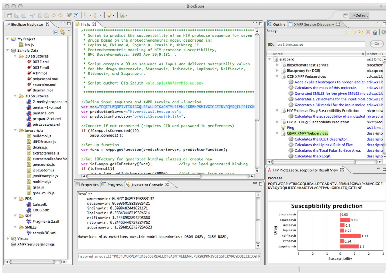
Figure 3 XMPP services used from Bioclipse. Screenshot from Bioclipse with the HIVpred plugin installed. The Bioclipse Console (bottom) was used to invoke the HIVpred service, and the results are displayed in this console and graphically in a chart (bottom right). In the top middle is shown a script making use of the HIVpred service for pipelined usage. The Service Discovery View displays the available services on the server ws1.bmc.uu.se (top right).
