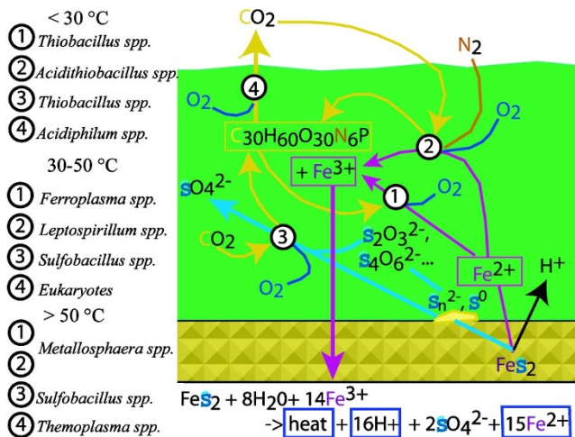
FIG. 9. Schematic diagram of microbial metabolisms prevalent at the Richmond Mine study site.
