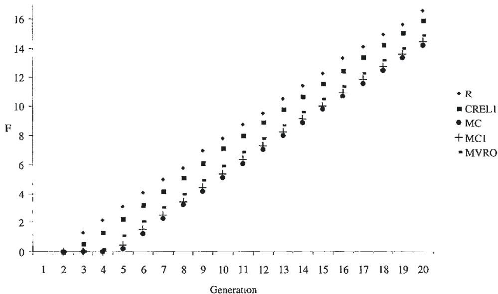
Figure 1. Coefficient of inbreeding ( F ) for schemes where \Delta F was constrained to 1.0% per generation, the number of selection candidates was 100 and the heritability was 0.25. The F of the R1, C and CREL1 was always between F of the R (♦) and CREL1 (■) schemes and has been omitted to increase readability of the graph. R: Random, CREL1: Compensatory, MC and MC1: Minimum coancestry, MVRO: Minimum variance of relationship of offspring.
