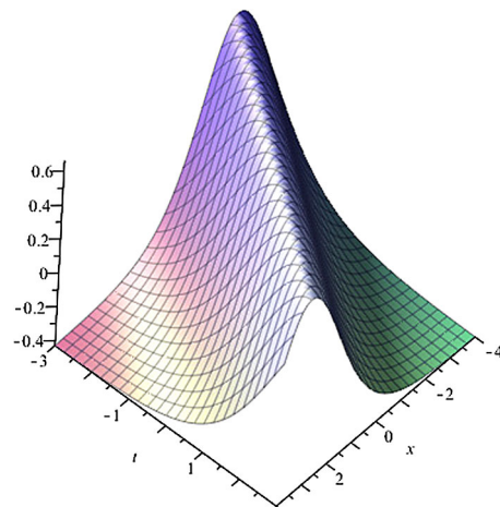
Figure 1 The solitary wave solution y_{33} of the KdV-Sawada-Kotera-Ramani equation (1.1) with a = 1, b = 1, and c = 1.
