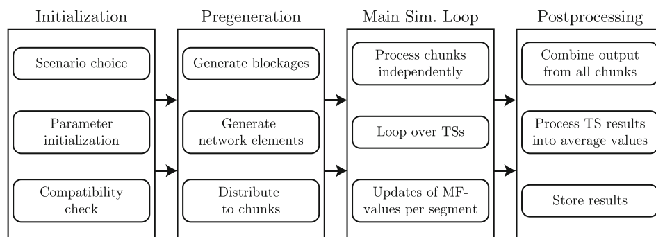
Fig. 1 Structure overview of the Vienna 5G SL simulator. The simulator is divided into four major blocks. In the figure, the main tasks that are performed per block are displayed
