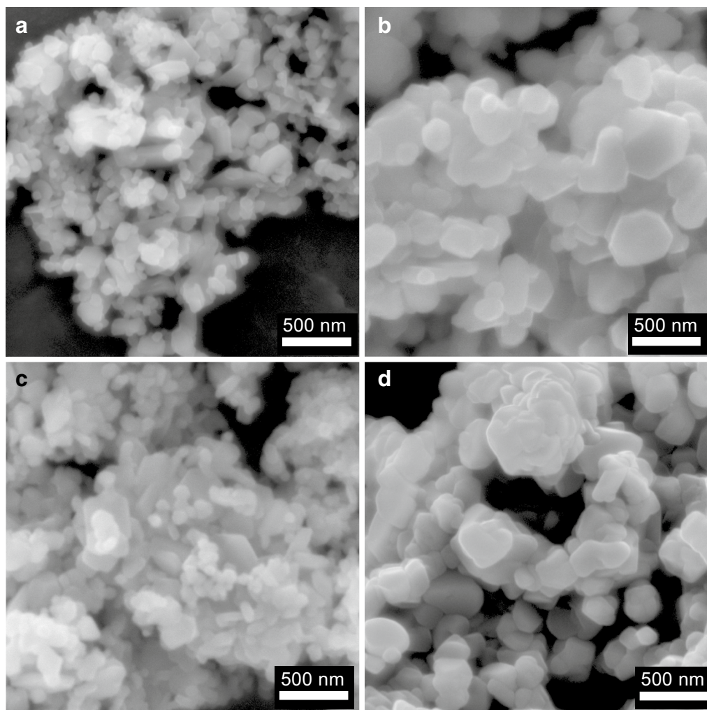
Fig. 11 SEM images of \text{LiCoO}_2 materials prepared with \text{LiO}^t\text{Bu} (a), \text{LiO}^i\text{Pr} (b), \text{LiOMe} (c), \text{LiOPh} (d) annealed at 600\text{ }^\circ\text{C}
