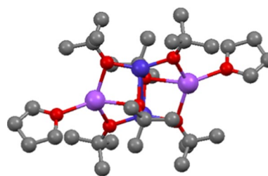
Fig. 3 Proposed structure for 8 (left) based on the [Na 2 Co 2 (O t Bu) 6 (thf) 2 ] compound (right, dark blue Co, violet Na, red O, grey C; H-atoms omitted described in [60])
