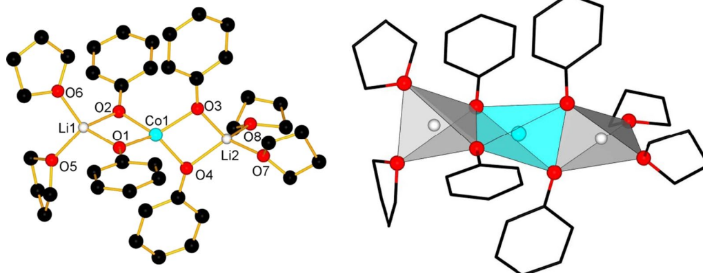
Fig. 2 Labelled view of the molecular structure of 1 , H-atoms are omitted for clarity (left); coordination polyhedra in 1 (right)
