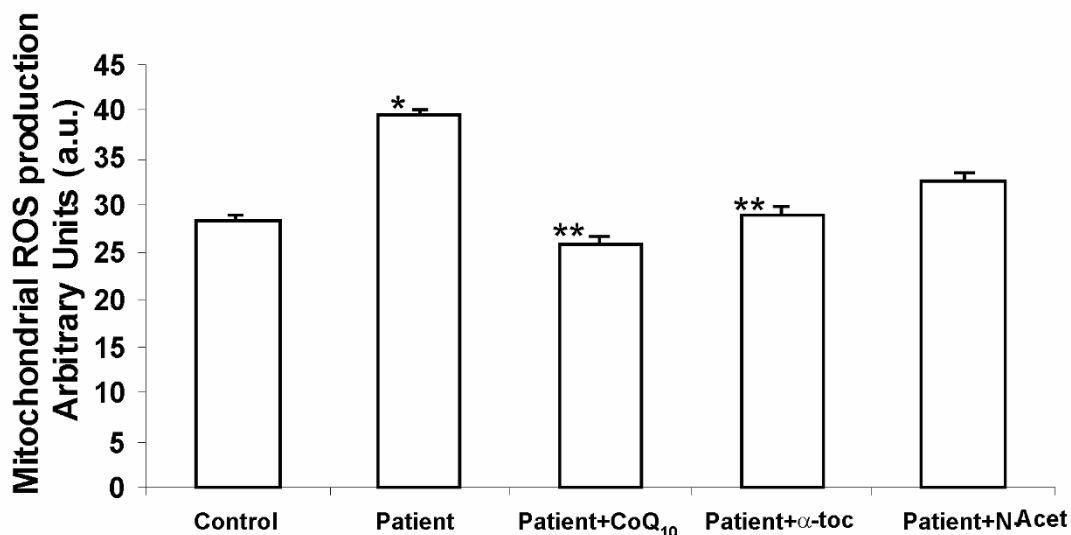
Figure 3 Effect of antioxidants on reactive oxygen species (ROS) generation. Blood mononuclear cells (BMCs) of representative fibromyalgia (FM) patients were treated with 10 \mu mol/L CoQ 10 , 30 \mu mol/L \alpha -tocopherol ( \alpha -toc), and 10 \mu mol/L N -acetylcysteine (N-Acet) for 24 h. Data represent the mean \pm SD of three separate experiments. * P < 0.001 between controls and FM patients; ** P < 0.005 between the absence or presence of CoQ 10 and \alpha -toc treatment.
