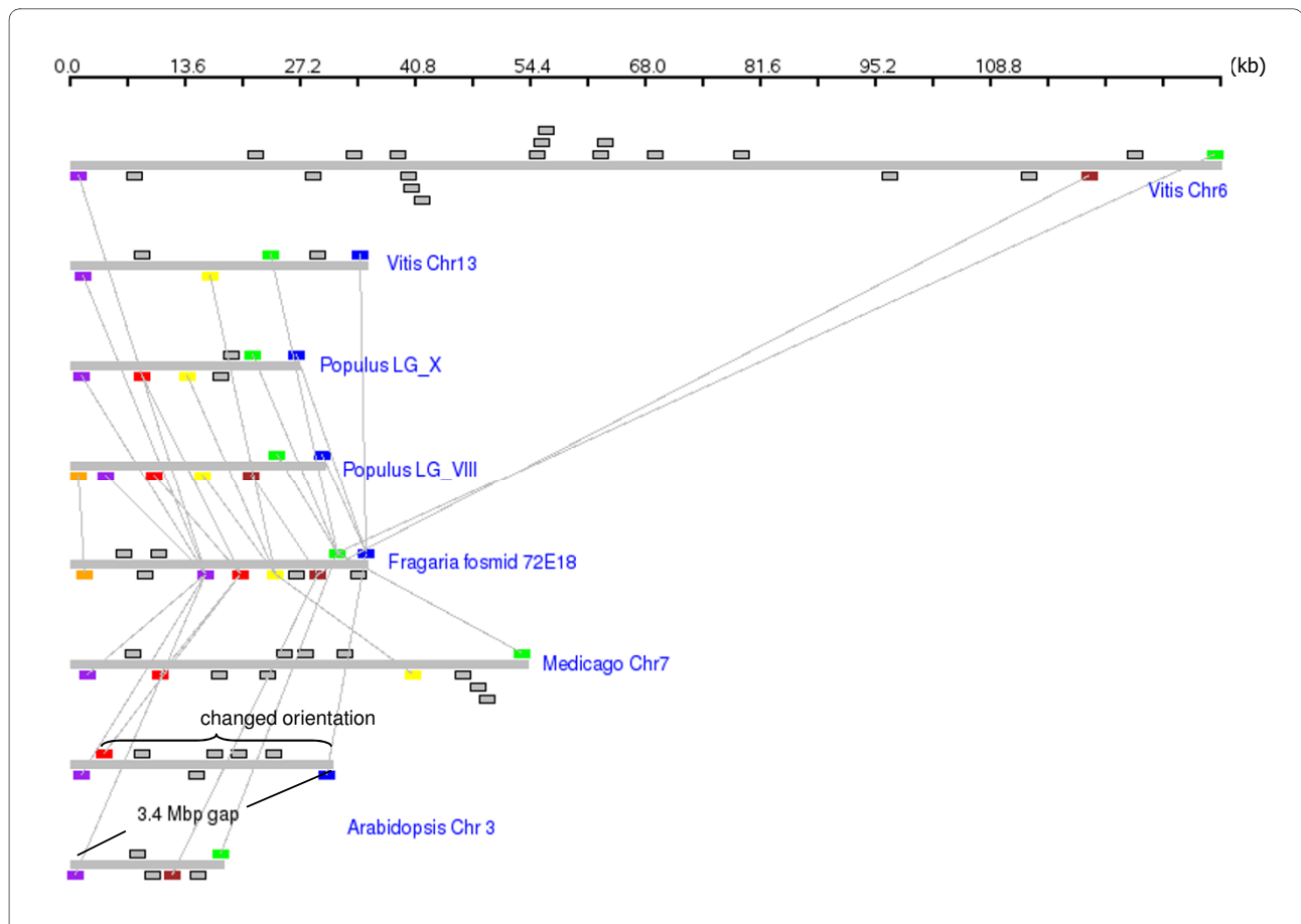
Figure 2 Conserved microsyntenic regions with Fosmid 72E18. The genomic segments are drawn according to their size but the genes are drawn with the same generic size. Squares above the lines represent genes located on the Crick strand and those below the lines represent genes on the Watson strand. Genes with the same color represent homologs and the gray squares represent genes without homologs in the genomic regions shown. Vitis Chr6, Populus LG_VIII, Medicago Chr7, and Arabidopsis genomic segments are drawn 3' to 5' and the rest are 5' to 3'. The diagram is drawn using GenomePixelizer [31].
