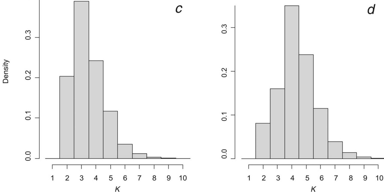
Figure 2 Estimated number of populations from Structure (a and b) and Geneland (c and d) analyses. Structure analyses: (a) mean ( \pm SD) probabilities of the data [ \ln Pr(X|K) ] over 10 Structure replicated runs plotted as a function of the putative number of clusters ( K ). (b) Mean variations of probabilities of the data ( \Delta(\ln Pr(X|K)) ) between successive K considered in Structure analyses. For K clusters, this variation is calculated as \Delta(\ln Pr(X|K)) = \ln Pr(X|K)_{k+1} - \ln Pr(X|K)_k . Geneland analyses: posterior density distribution of the number of clusters estimated from Geneland analysis in 7 out of 10 replicates (c) and in the 3 remaining trials (d).
