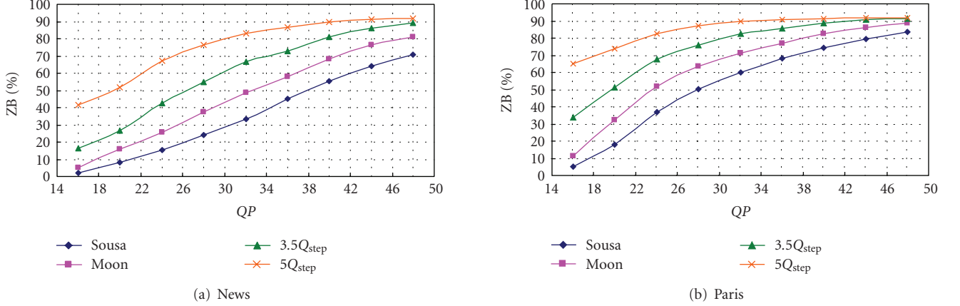
FIGURE 2: Zero-block detecting capability.
