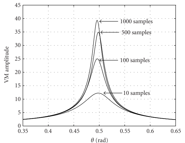
FIGURE 7: Vector MUSIC for different sample numbers.
