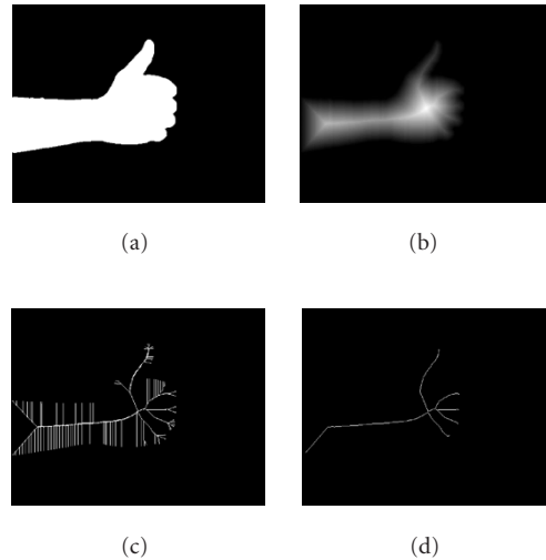
FIGURE 6: Skeleton extraction: (a) hand region (binary image), (b) chamfer distance image (white corresponds to the greatest distance), (c) the skeleton obtained after connecting the centers of maximal discs, and (d) the skeleton obtained after spurious hole filling, pruning, and beautifying the previous skeleton.
