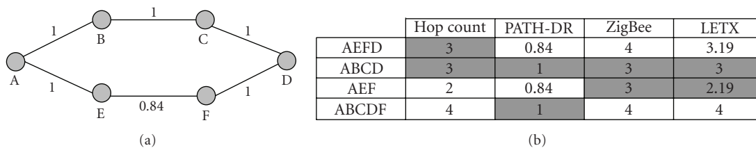
FIGURE 15: Example of route selection based on LETX and ZigBee metrics, whereby PDR grows as the distance between sender and receiver grows. The number placed next to a link indicates the LDR of that link. The shaded boxes indicate the cost of the path selected by each routing metric between node A and nodes D and F.
