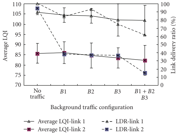
FIGURE 21: Influence of background traffic on LQI and LDR for two different links in scenario A. For the LQI, the standard deviation intervals are depicted.
