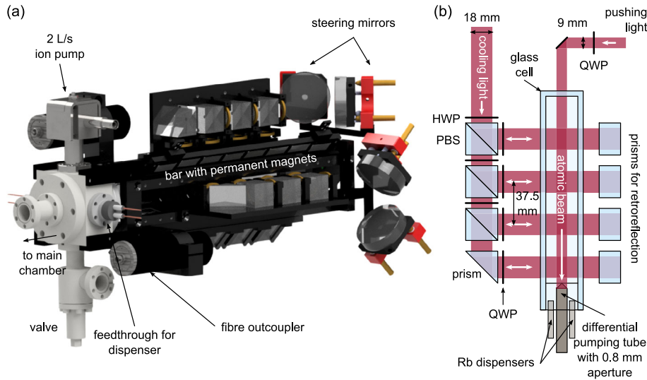
Fig. 1. 2D MOT setup. (a) Overview. All optics and magnets required are mounted on a cage structure surrounding a ultra-high vacuum glass cell. Dispenser feed-throughs, valves, an ion pump, and the cell attach to a square metal block. (b) Optical setup. The cooling light is divided into circularly polarised beams for four separate cooling regions using a combination of polarising beam splitters (PBS) and half and quarter wave plates (HWP/QWP). A circularly polarised pushing beam is co-propagating on the atomic beam axis. The beam sizes given correspond to the respective 1/e^2 diameters.
