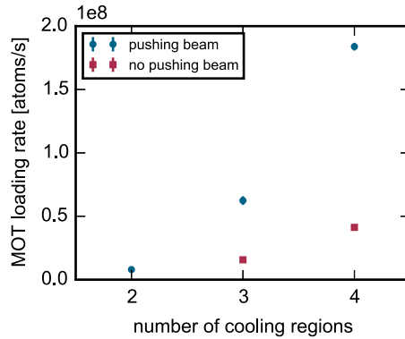
Fig. 2. Influence of cooling volume size on 2D MOT performance. The MOT loading rate is shown as different numbers of cooling regions are used comparing the performance with (blue circles) and without (red squares) use of the pushing beam.
