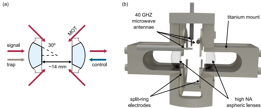
Fig. 3. In-vacuum lens assembly. The mount for the high NA aspheric lenses (effective focal length \approx 10.3 mm) was milled from a single titanium block. A set of split ring electrodes as well as three simple microwave antennae rated up to 40 GHz made from open ended SMA-K cable were incorporated into the assembly. Macor holders for the antennae and a pair of anti-Helmholtz coils generating the magnetic gradient field the MOT are not shown for simplicity. All titanium and Macor surfaces have been coated with a thin platinum layer to avoid the built-up of patch charges.
