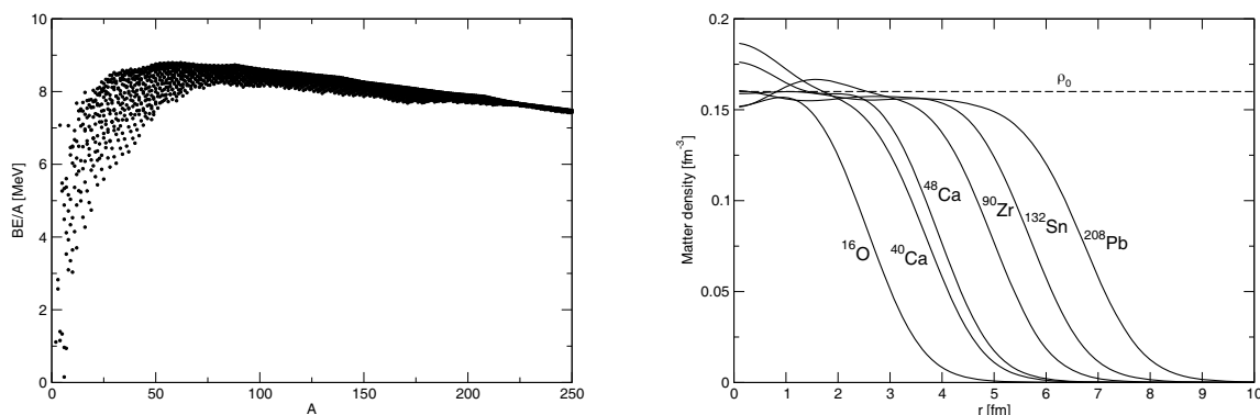
Fig. 2. (Left panel) Binding energy per particle B/A as a function of the mass number A (data from refs. [1,2]). (Right panel) Nuclear matter density for few nuclei. The horizontal line marks the saturation density.
