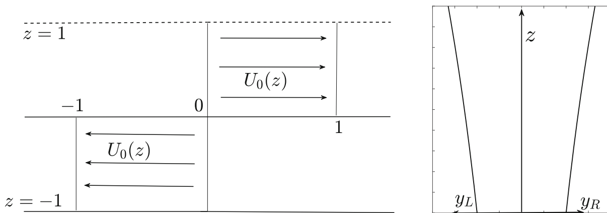
Fig. 2. Velocity profile and width function of the channel: (a) Bounded vortex sheet with a free upper surface; (b) topography.
