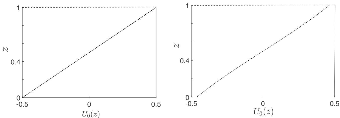
Fig. 1. Velocity profiles in examples 1 and 2: (a) Velocity profile of U_0(z) = z - 1/2 ; (b) velocity profile of U_0(z) = \tanh(z - 1/2) .
