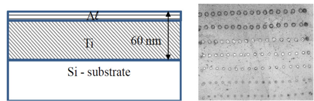
Fig. 1 Schematic views of the BMTF cross section and optical image after the single fs laser pulse irradiation (pulse duration 300 fs, wavelength 515 nm, pulse energy from 0.03 to 0.48 \mu\text{J} )
