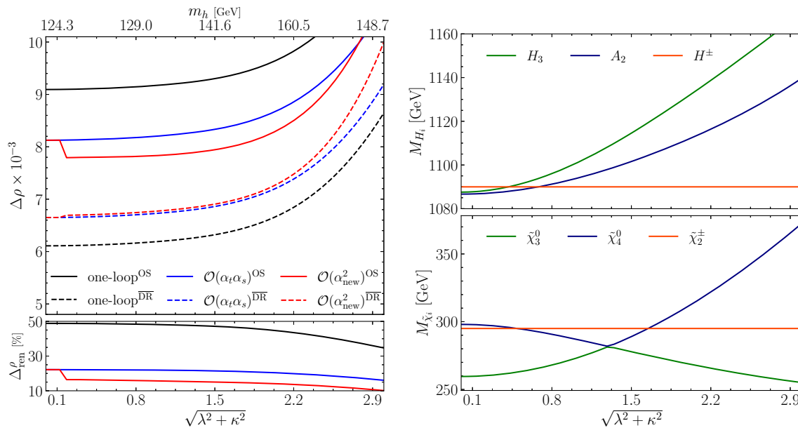
Fig. 1 Upper left: the \rho parameter at full one-loop order (black), two-loop \mathcal{O}(\alpha_t \alpha_s) (blue) and two-loop \mathcal{O}(\alpha_{\text{new}}^2) (red) as function of \sqrt{\lambda^2 + \kappa^2} . The dashed lines are for the \overline{\text{DR}} scheme in the top/stop sector while the full lines are for the OS scheme. Lower left: renormalization scheme dependence \Delta_{\text{ren}}^\rho of the \rho parameter at full one-loop order (black), at two-loop \mathcal{O}(\alpha_t \alpha_s) (blue) and \mathcal{O}(\alpha_{\text{new}}^2) (red).
