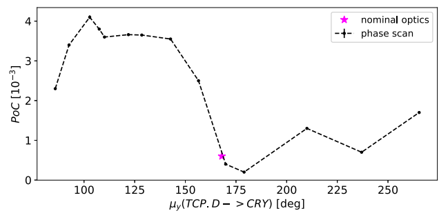
Fig. 5 The dependence of the fraction of the number of protons impacting the crystal over the number of protons impacting the primary collimator (PoC) on the betatron phase from the primary vertical collimator in IR7 (TCP.D) to the IR2 crystal (CRY). Crystal retraction is 7.9 \sigma . Statistical errors are on the order of 1%, which makes the bars hardly visible
