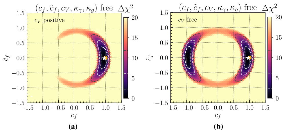
Fig. 8 Fermion-vector model: results of fits to the LHC measurements in the (c_f, \tilde{c}_f) parameter plane. The coupling modifiers c_f, \tilde{c}_f, \kappa_\gamma, \kappa_g are free-floating in both plots, while a c_V is restricted to positive values and b c_V is free-floating. In each case, the \mathcal{CP} -even and \mathcal{CP} -odd parts of the couplings shown in the plot are free-floating while all the other parameters are set to their SM values. The legend corresponds to the one in Fig. 2
