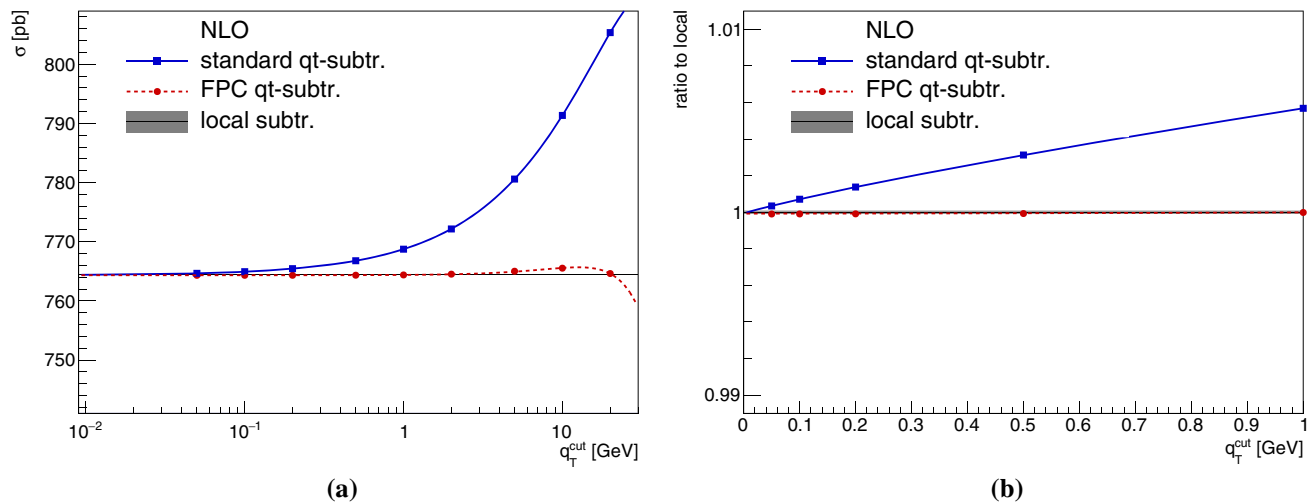
Fig. 1 Fiducial cross section for the production of l^+l^- pairs from Z/\gamma^* decay at the LHC ( \sqrt{s} = 13 TeV). NLO results with the q_T subtraction method (blue squared points) and q_T subtraction method
