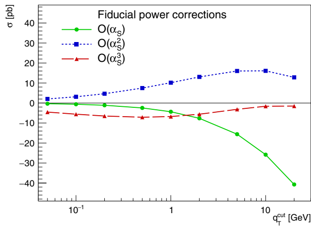
Fig. 4 Production of l^+l^- pairs from Z/\gamma^* decay at the LHC ( \sqrt{s} = 13 TeV). Power correction contributions at \mathcal{O}(\alpha_S) , \mathcal{O}(\alpha_S^2) and \mathcal{O}(\alpha_S^3) at various values of q_T^{\text{cut}}
