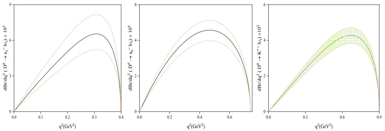
Fig. 3 Differential branching ratios of the D^0 \rightarrow K^{*-} \ell \nu_\ell , D^0 \rightarrow a_1^- \ell \nu_\ell and D^0 \rightarrow a_0^- \ell \nu_\ell as functions of q^2
