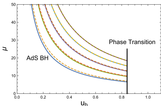
Fig. 7 The tensor glueball spectrum (dashed line) in the AdS BH sector, i.e., below the horizon, as a function of u_h , compared with that of scalar glueballs (solid lines)
