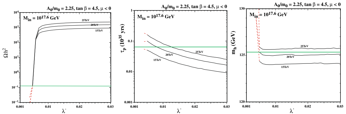
Fig. 12 As in Fig. 6, as functions of \lambda' for the indicated fixed values of m_{1/2} \in [15, 25] TeV and m_0 chosen to obtain the cosmological value of \Omega_{\text{LSP}} h^2 for \lambda_\Theta = 0.005 , with the same values of the other input parameters as in Fig. 3
