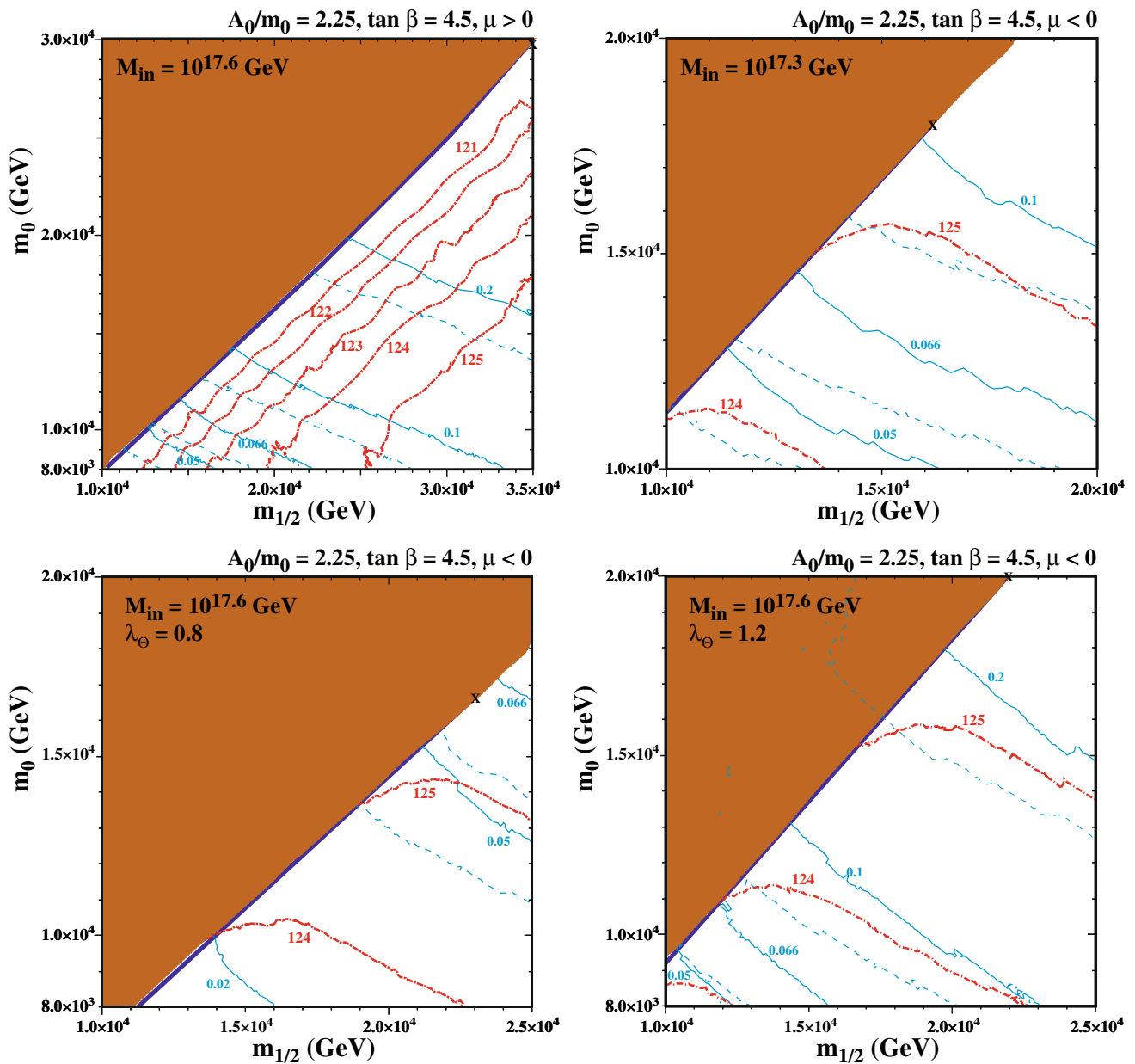
Fig. 4 Upper left panel: the (m_{1/2}, m_0) plane for the parameters \tan \beta = 4.5 , A_0 = 2.25m_0 , B_0 = 1.25m_0 , M_{\text{in}} = 4 \times 10^{17} GeV, M_\Theta = 3 \times 10^{17} GeV, \lambda' = 0.005 and \lambda_\Theta = 1 with \mu > 0 . Upper right panel: The corresponding plane with M_{\text{in}} = 2 \times 10^{17} GeV, \mu < 0 and unchanged values of the other parameters. Lower panels: the corre-
