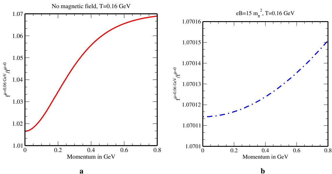
Fig. 1 Variations of the ratio of quark distribution function at \mu = 0.06 GeV to its value at \mu = 0 with momentum at low temperature in the a absence and b presence of strong magnetic field
