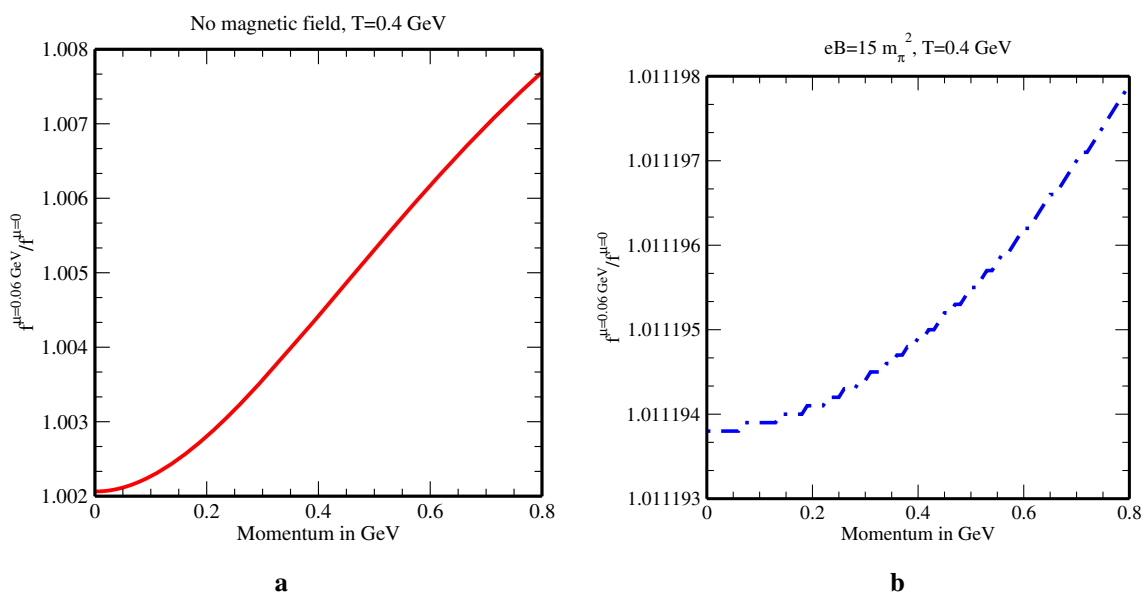
Fig. 2 Variations of the ratio of quark distribution function at \mu = 0.06 GeV to its value at \mu = 0 with momentum at high temperature in the a absence and b presence of strong magnetic field
