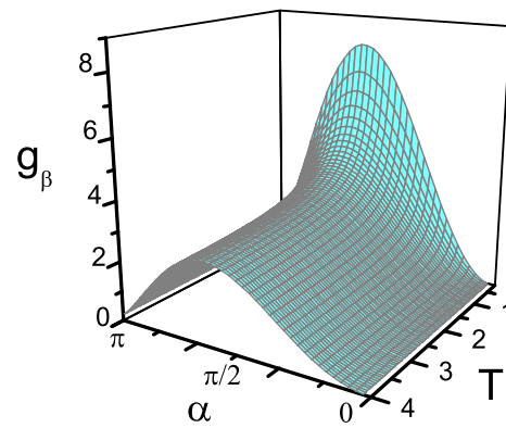
Fig. 4 The quantum parameter estimation with respect to \beta is evaluated by \mathcal{G}_\beta as a function of the amplitude \alpha and radiation temperature T when the frequency of Dirac field \omega = 1 is chosen
