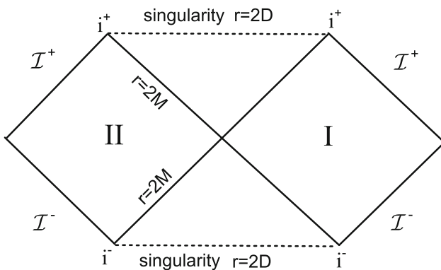
Fig. 1 The Penrose diagrams for the GHS dilation black hole can be illustrated
