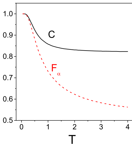
Fig. 5 The decoherence of quantum coherence C and quantum Fisher information \mathcal{F}_\alpha are illustrated by the black line and red dash line respectively. The parameters of \alpha = \pi/2 and \omega = 1 are chosen
