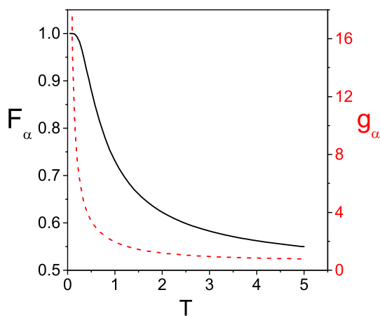
Fig. 3 The decoherence of \mathcal{F}_\alpha and \mathcal{G}_\alpha is illustrated by the black line and red dash line respectively. The parameters of \alpha = \pi/4 and \omega = 1 are chosen
