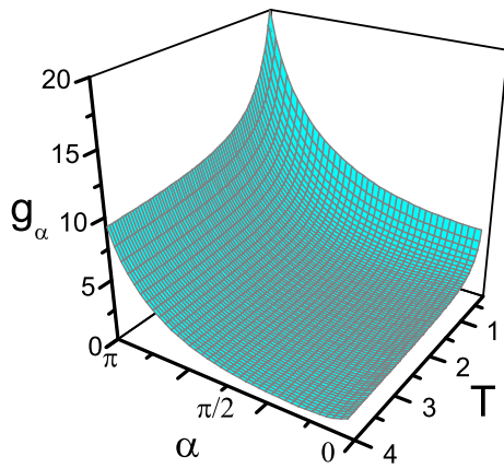
Fig. 2 The quantum parameter estimation with respect to \alpha is evaluated by \mathcal{G}_\alpha as a function of radiation temperature T when the frequency of Dirac field \omega = 1 is chosen
