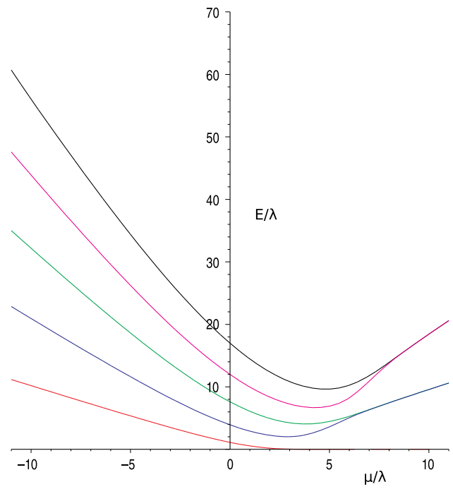
Fig. 2 Plot of the universal ratio E/\lambda for the first five eigenvalues as functions of \mu/\lambda from -11 to +11
