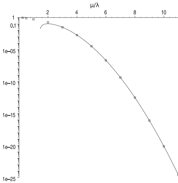
Fig. 4 Logarithmic plot of the ratio E_1/\lambda for the first eigenvalue N = 1 as a function of positive \mu/\lambda . The solid line shows theoretical value, small squares mark computed numerical values
