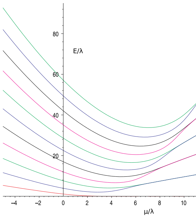
Fig. 1 Plot of the universal ratio E/\lambda for the first 11 eigenvalues as functions of \mu/\lambda from -5 to +11
