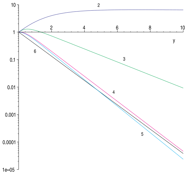
Fig. 5 Full propagators for different values \mu and \lambda as functions of y . (2) \mu = 1 , \lambda = 1/3 ; (3) \mu = 1 , \lambda = 1 ; (4) \mu = 0.1 , \lambda = 1 ; (5) \mu = 0 , \lambda = 1 ; (6) \mu = -1 , \lambda = 0.1
