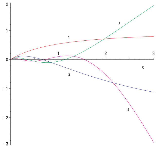
Fig. 3 Plot of the first four eigenfunctions for the case \mu = 0.1, \lambda = 1 at small x
