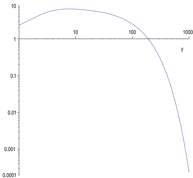
Fig. 6 Full propagator for \mu = 1 and \lambda = 1/3 as a function of y with both axes given in the logarithmic scale
