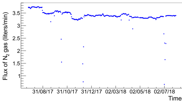
Fig. 37 Evolution of the nitrogen gas flux entering into the ANAIS-112 shielding to prevent radon intrusion, averaged per day
