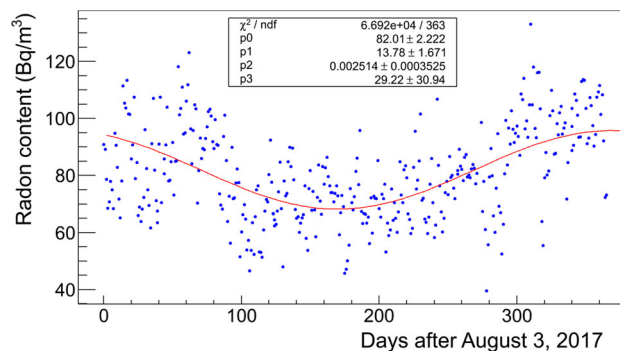
Fig. 36 Evolution of the radon content in the LSC hall B air in the ANAIS hut outside the shielding. Rates are calculated per day and fitted to a cosinoidal dependence
