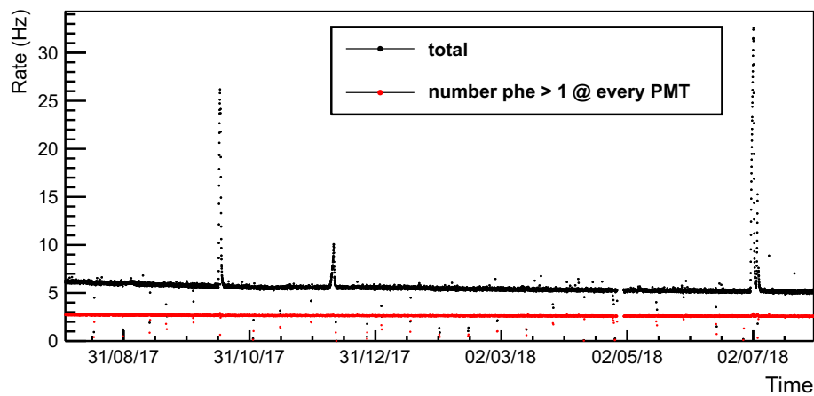
Fig. 5 Trigger rate (calculated in 3600 s time bins) during the first year of ANAIS-112 DM data taking: total trigger rate is shown in black, trigger rate of events having more than one phe in the pulse at each PMT is shown in red. Strong increases in the total trigger rate of the experiment are related with exhausting the liquid nitrogen dewar providing
