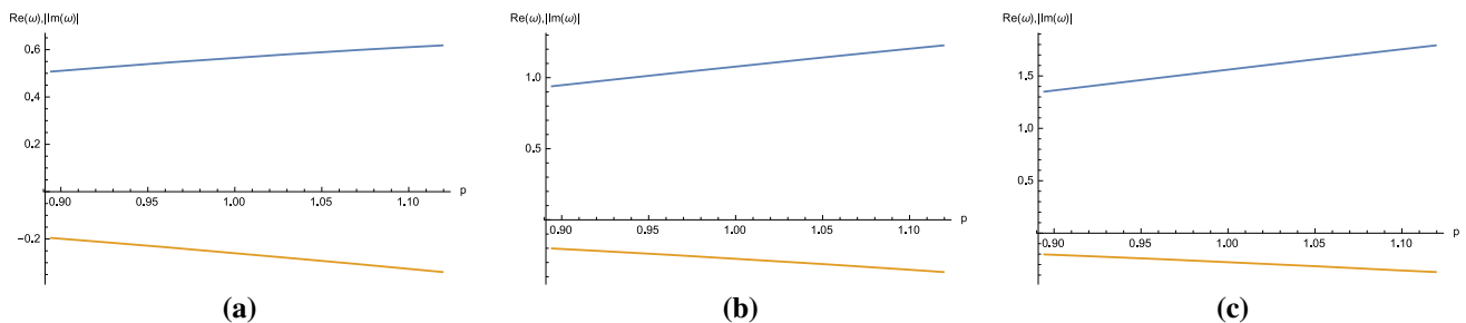
Fig. 2 The fundamental quasinormal mode ( n = 0 ) for the electromagnetic field ( s = 1 ), blue line is real part of frequencies, orange line is imaginary part: a l = 1 ; b l = 2 ; c l = 3
