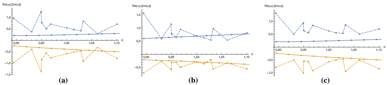
Fig. 1 The fundamental quasinormal mode ( n = 0 ) for the scalar field ( s = 0 ), blue line is real part of frequencies, red line is imaginary part; dashed lines are the data obtained in the work [23], positive values for the real part and negative values for the imaginary part: a l = 0 ; b l = 1 ; c l = 2
