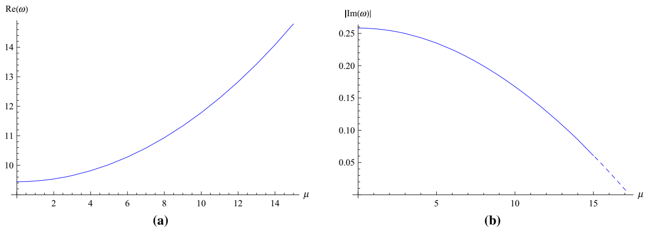
Fig. 3 Dependence of frequency components on mass \omega(\mu) with s = 0 , l = 20 , p = 1 , \mu = 0 \dots 16 : a \text{Re}(\omega) ; b absolute value of \text{Im}(\omega)
