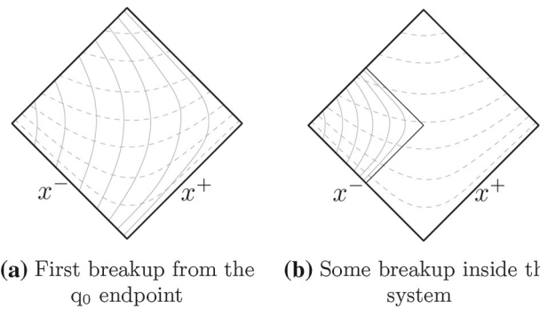
Fig. 4 Hyperbolae of constant \Gamma and m_h^2 represented by dashed and full lines, respectively
