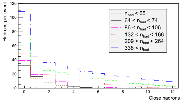
(b) Excluding adjacent hadrons
