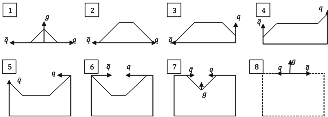
Fig. 6 Time evolution of the qq\bar{q} system formed by massless partons in a frame where the gluon moves in the +x direction, while the q and \bar{q} move in opposite directions along the z axis
