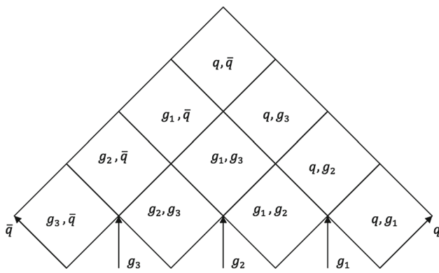
Fig. 11 Parameter plane for a five parton system
