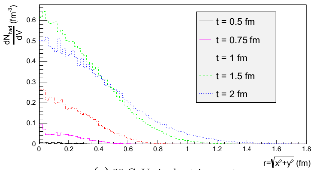
(a) 20 GeV single string systems
