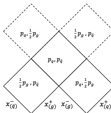
Fig. 7 The parameter plane picture for the qq\bar{q} system. The dash lines indicate the turnover regions, normally neglected
