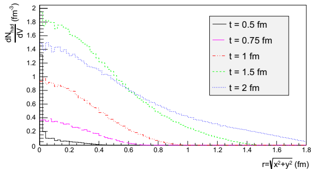
(b) 13 TeV pp collisions
