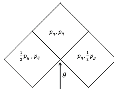
Fig. 10 Parameter plane for a q\bar{q}g system
