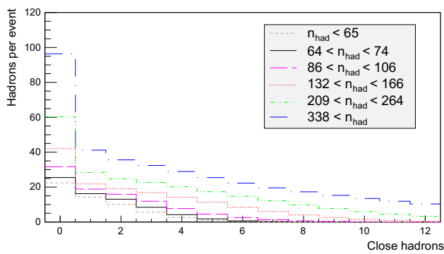
(a) Including adjacent hadrons
