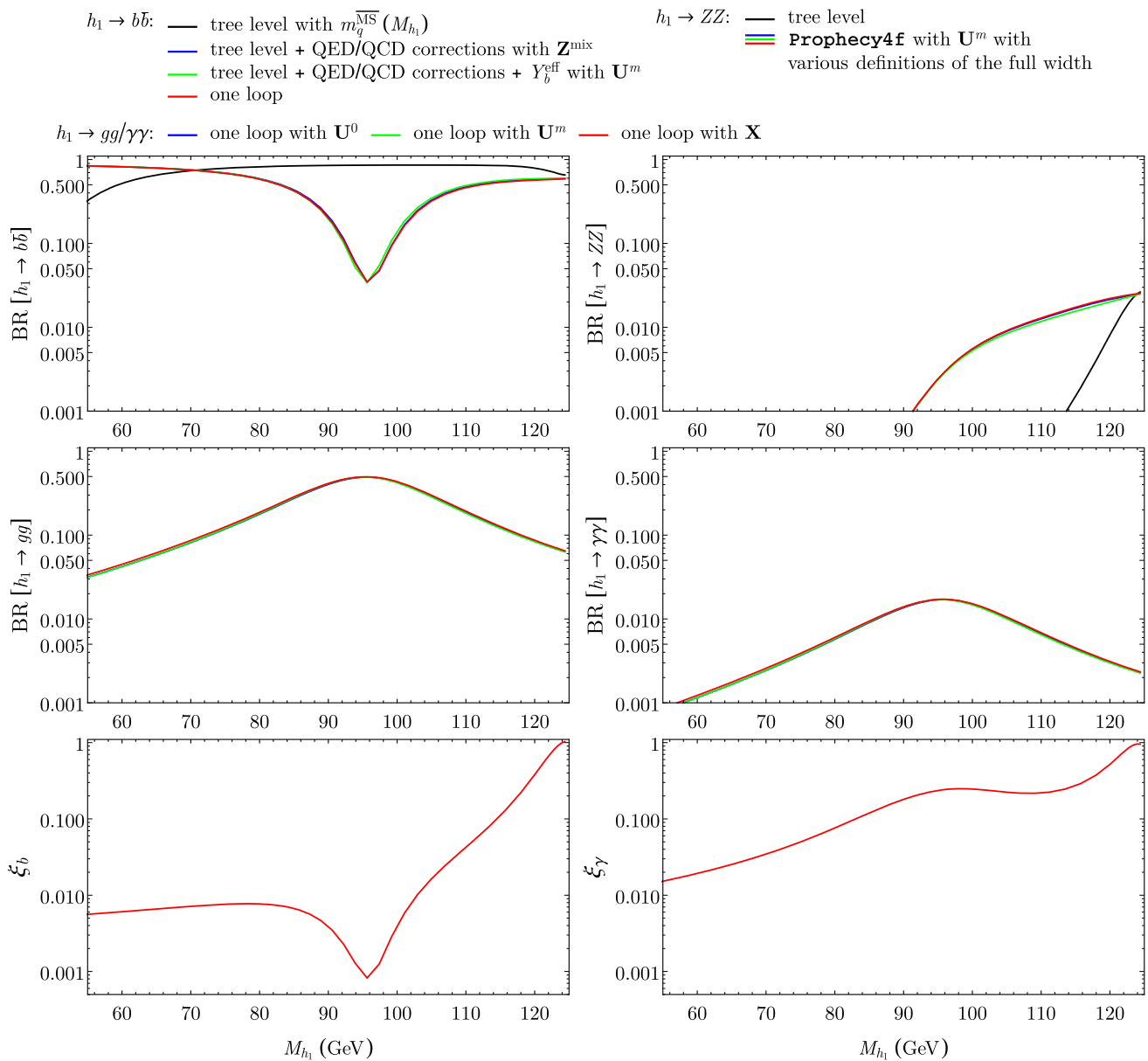
Fig. 13 The decay properties of the mostly singlet CP -even Higgs state as a function of its mass are shown. The input parameters are provided in Table 1. The branching ratios into b\bar{b} , ZZ , gg and \gamma\gamma are shown at the tree level (black), under partial one-loop approximations (blue, green) or at the full one-loop order (red). The plots at the bottom show the quan-
