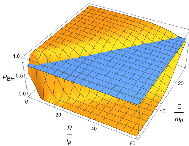
Fig. 6 Probability for two collapsing shells with momenta P_1 = -5P and P_2 = -P to form a black hole as a function of the radius R and the total energy E (in Planck units). The blue plane delimits the region where the probability P_{\text{BH}} > 0.8
