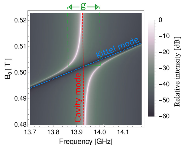
Fig. 1 Transmission spectrum of the hybrid system as a function of the external field B_0 , showing the anticrossing curve of the cavity mode (red dashed line) and Kittel mode (blue dashed line). The coupling g is defined by Eq. (5)
