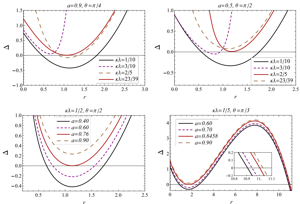
Fig. 2 Plot showing the variation of \Delta with r for different values of parameter \kappa\lambda and a for black hole ( M = 1, Q = 0.2 ) surrounded by dust field. (Red solid curve) corresponds to the extremal black hole
