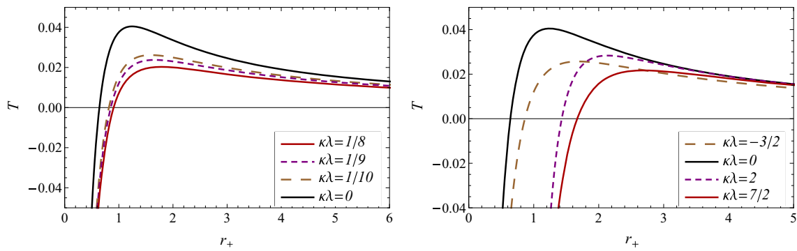
Fig. 6 Plot showing the variation of Hawking temperature T with horizon radius r_+ for different values of Rastall coupling \kappa\lambda for rotating Rastall black hole ( a = 0.5, Q = 0.1 ) surrounded by dust (left) and quintessence field (right). (Black solid curve) represent the temperature profile for KN black hole in vacuum
