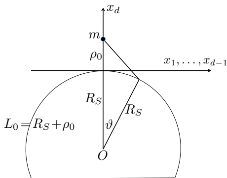
Fig. 1 The initial position of the test mass m . O is the center of the spherical horizon of radius R_S
