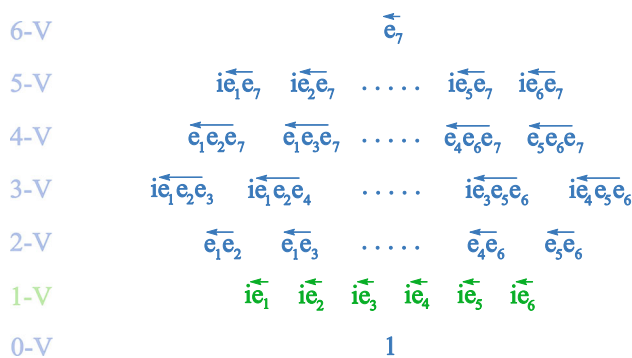
Fig. 3 The left action of \mathbb{C} \otimes \mathbb{O} on itself provides a faithful representation of Cl(6) , and is hence isomorphic to the 8 \times 8 \mathbb{C} matrices. Here, left-action maps, i \overleftarrow{e}_j , for j = 1, \dots, 6 , form the generating space (1-vectors)
