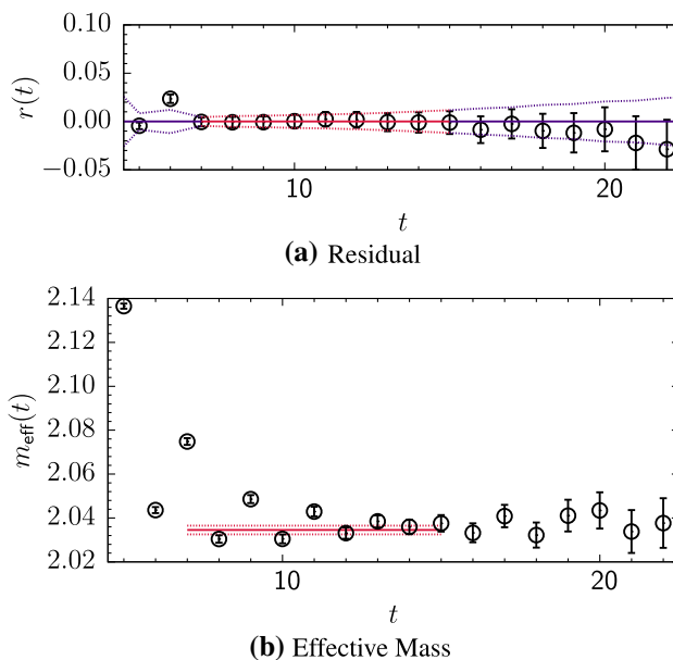
Fig. 1 Correlated fit results for a pseudoscalar heavy-light meson correlator generated with the OK action at \kappa = 0.041 and \mathbf{p} = \mathbf{0} . a Residual defined in Eq. (29) and its statistical error from a fit over 7 \leq t \leq 15 ; the kinks for t < 7 are a remnant of the oscillating, wrong-parity states, seen in the right-hand side of Eq. (25). b Effective mass (points) defined in Eq. (28) with fit result for the ground-state energy E (horizontal red line plotted over the chosen fit interval)
