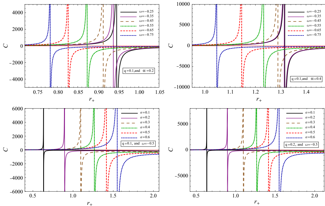
Fig. 4 The specific heat ( C_+^{\text{EGB}} ) vs. horizon radius r_+ for the 5D Einstein–Gauss–Bonnet black hole surrounded by the quintessence matter for different values of \omega and \alpha
