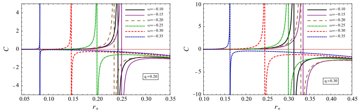
Fig. 5 The specific heat ( C_+ ) vs. horizon radius r_+ for the 5D general relativity black hole surrounded by the quintessence matter. The black hole thermodynamically unstable when C_+ < 0 , and stable when C_+ > 0
