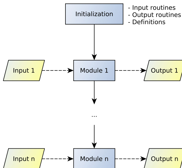
Fig. 1 DsixTools 's global flowchart. The user can provide input to each module or use the results obtained with the previous one
