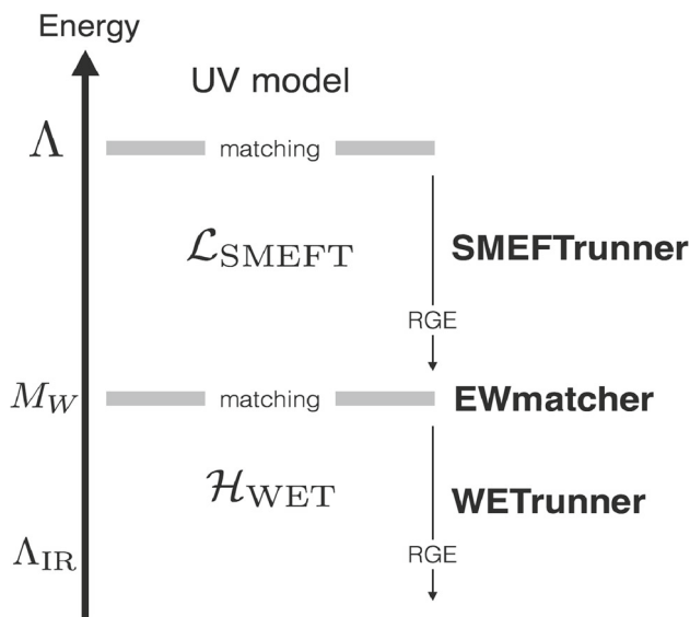
Fig. 2 Functionality of DsixTools modules
