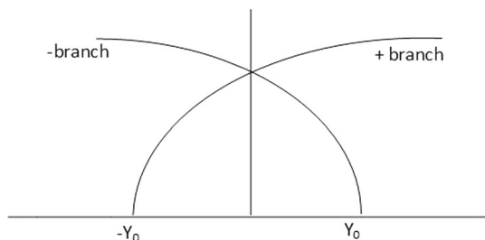
Fig. 3 Non-singular matching solution for C > 0, k > 0 and \gamma > -1/2 . We take the (+) branch for Y > 0 and the (-) branch for Y < 0
