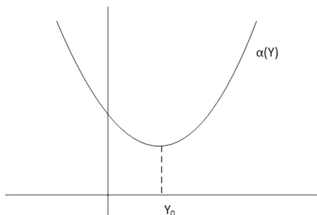
Fig. 1 Non-singular solution for C < 0, k > 0 and \gamma > -1/2 , or C > 0, k < 0 and -1 < \gamma < -1/2
