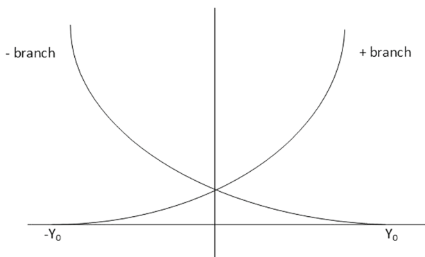
Fig. 2 Non-singular matching solution for C > 0, k > 0 and -1 < \gamma < -1/2 . We take the (+) branch for Y > 0 and the (-) branch for Y < 0
