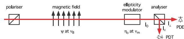
Fig. 1 A simple heterodyne ellipsometer. PDE extinction photodiode, PDT transmission photodiode
