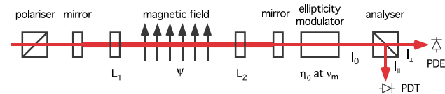
Fig. 3 Proposed modulation scheme. L_{1,2} rotating half-wave-plates, PDE extinction photodiode, PDT transmission photodiode
