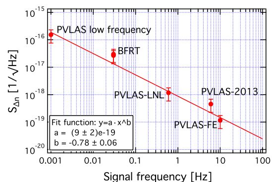
Fig. 2 Birefringence noise densities measured in polarimeters set up to measure the magnetic vacuum birefringence plotted as function of the frequency. Data from the experiments BFRT [20], PVLAS-LNL [21, 22], PVLAS-2013 [23], PVLAS-FE [12] are normalised to the length of the optical cavities, to the number of passes and to the wavelength. The leftmost point has been measured during the 2015 data taking campaign of the PVLAS experiment. The two almost equivalent points from BFRT are measured with two different cavities, one having 34 passes and the other 578 passes. The error bars are an estimated 50 %
