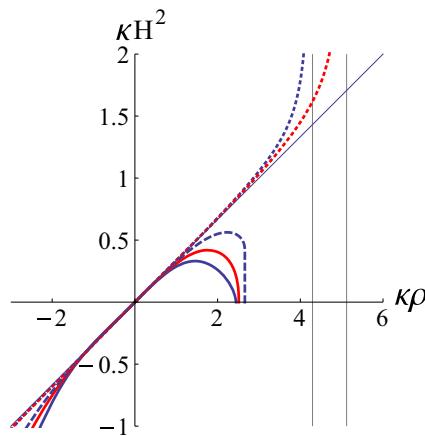
Fig. 3 Graphical representation of \kappa H^2 as a function of \kappa\rho for a radiation dominated universe ( w = 1/3 ). Different curves represent different values of \beta . The solid blue, red, dashed blue, dotted blue, and dotted red curves show the representations for \beta = 1/10, 3/25, 7/50, 1/5, and 21/100 , respectively. The straight line crossing the origin represents H^2 = \rho/3 , which is the solution within R + R^2 gravity ( \beta = 1/4 ) for a radiation dominated universe. Note that the vertical lines (from left to right) indicate the maximum values of the energy density for \beta = 1/5 and 21/100 , where the Hubble rate blows up, respectively. These singular events correspond to a big freeze singularity in the past
