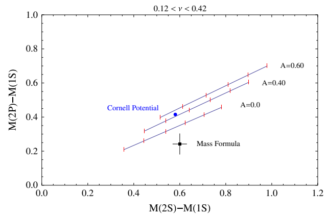
Fig. 1 Results for the mass differences in the plane M(2S) - M(1S) and M(2P) - M(1S) (in GeV). The squared box with errors corresponds to the eigenvalue differences estimated in (18). Lines indicate the results computed with fixed A and varying \nu . The round dot represents the result for the Cornell potential with charmonium parameters given in Eq. (10)
