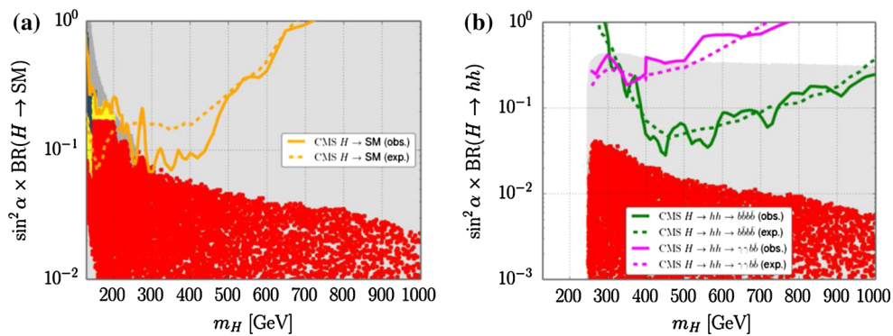
Fig. 12 Collider signal rates of the heavy Higgs boson H decaying into SM particles (a) or into two light Higgs bosons, H \rightarrow hh (b) , in dependence of the heavy Higgs mass, m_H . The rates are normalized to the inclusive SM Higgs production cross section at the corresponding mass value [35, 101, 102]. a Heavy Higgs signal rate with SM particles in the final state. The orange solid (dashed) curves indicate the
