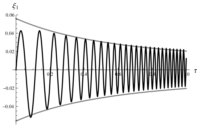
Fig. 1 Oscillations of \xi_1(\tau) , in the case n = 2, \kappa = 0.01, g = 0.01 and initial conditions y_0 = 1, y'_0 = \kappa/2 . The amplitude of the oscillations is in very good agreement with analytical estimate (12)
