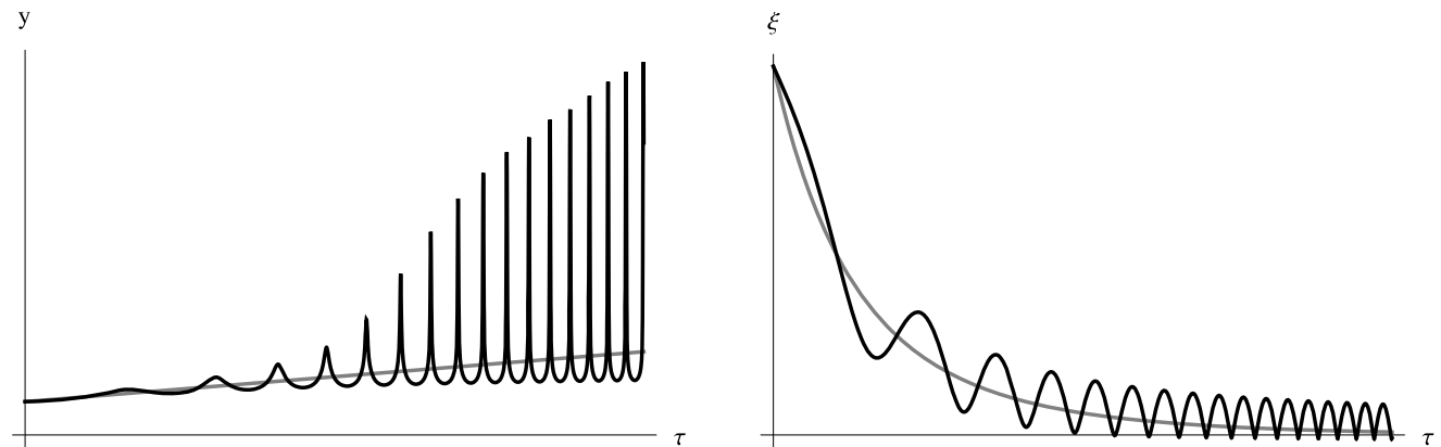
Fig. 2 “Spikes” in the solutions. The results presented are for n = 2, g = 0.001, \kappa = 0.4 , and y'_0 = \kappa/2 . Note the asymmetry of the oscillations of y around y = z and their anharmonicity
