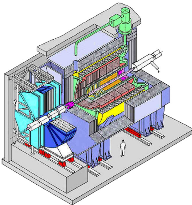
Fig. 30 The H1 detector at HERA. Source: H1
