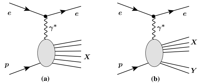
Fig. 1 Inclusive (a) and diffractive (b) deep inelastic scattering
