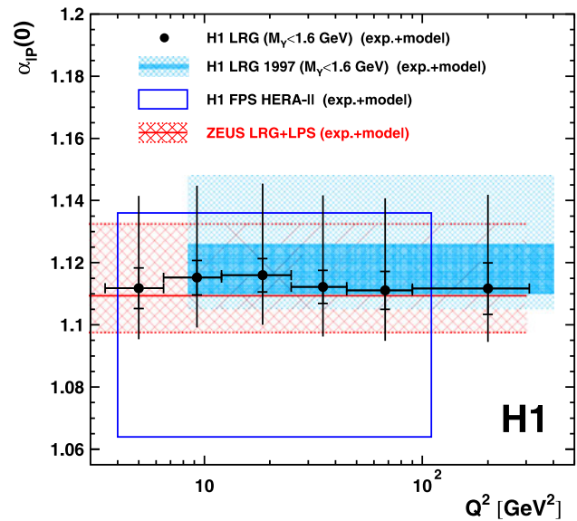
Fig. 12 Pomeron intercept values obtained from Regge fits in different Q^2 bins, as defined in the text (dots). The inner error bars represent the statistical and systematic errors added in quadrature and the outer error bars include model uncertainties in addition (see text for details). Previous determinations of the Pomeron intercept [10–12, 14] are also displayed for comparison. For these previous results the bands or boxes represent the combination of experimental and model uncertainties, always dominated by the model error
