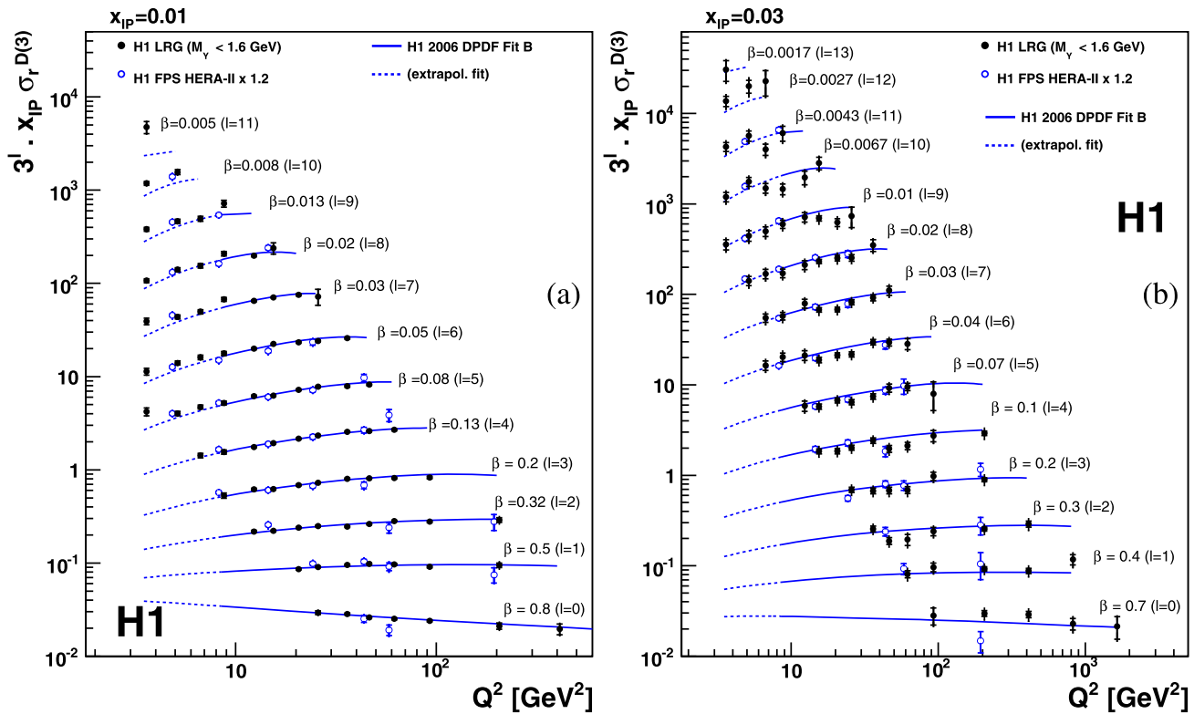
Fig. 9 The reduced diffractive cross section from combined H1 LRG data, multiplied by x_{\mathbb{P}} , at two fixed values of x_{\mathbb{P}} = 0.01 (a) and 0.03 (b). The reduced cross section values are multiplied by a scaling factor 3^l , with l values as indicated in parentheses. The LRG data are compared with the H1 FPS results [12] interpolated to the LRG \beta , Q^2 and x_{\mathbb{P}} values using a parametrisation of the H1 2006 DPDF Fit B [10].
