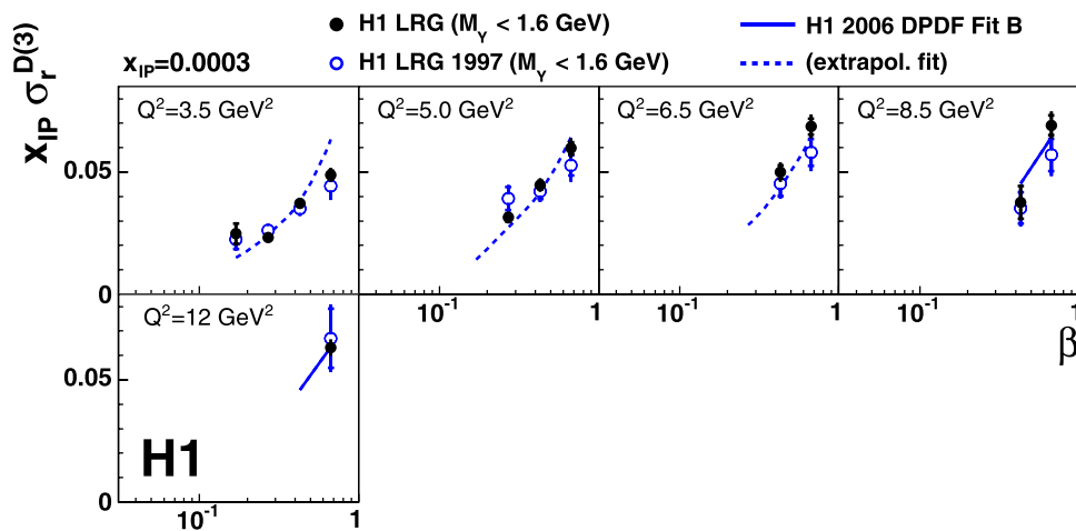
Fig. 3 The \beta dependence of the reduced diffractive cross section, multiplied by x_{\mathbb{P}} , at a fixed value of x_{\mathbb{P}} = 0.0003 , resulting from the combination of all data samples. Previously published H1 measurements [10] are also displayed as open points. The inner and outer error bars on the data points represent the statistical and total uncertainties, respectively.
