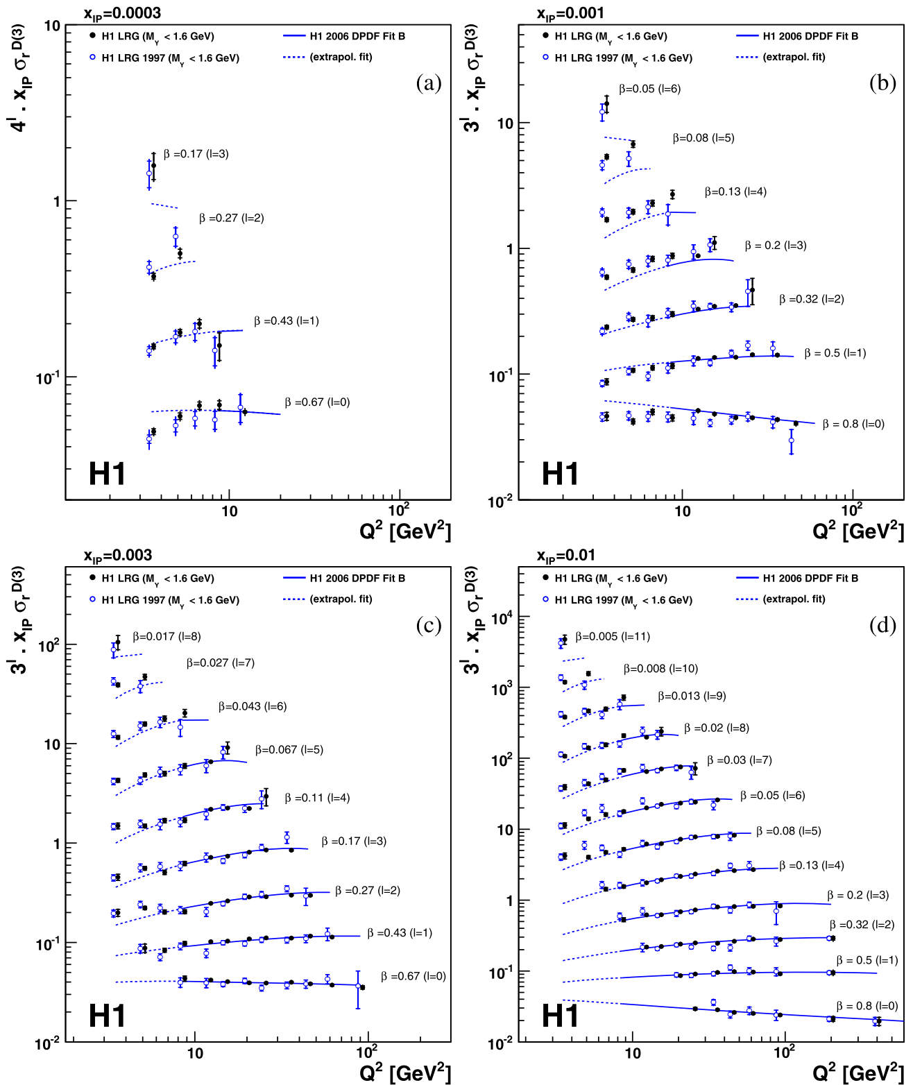
Fig. 7 The Q^2 dependence of the reduced diffractive cross section, multiplied by x_{IP} , at different fixed values of x_{IP} = 0.0003 (a), 0.001 (b), 0.003 (c) and 0.01 (d), resulting from the combination of all data samples. The reduced cross section values are multiplied by a scaling factor, 4^l for x_{IP} = 0.0003 and 3^l for x_{IP} = 0.003, 0.001 and 0.01, with
