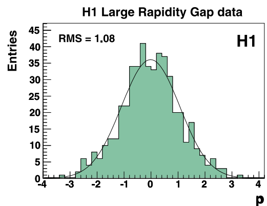
Fig. 2 Distribution of pulls p for all data samples. There are no entries outside the histogram range. The RMS gives the root mean square of the distribution calculated as \overline{p^2} . The curve shows the result of a binned log-likelihood Gaussian fit to the distribution
