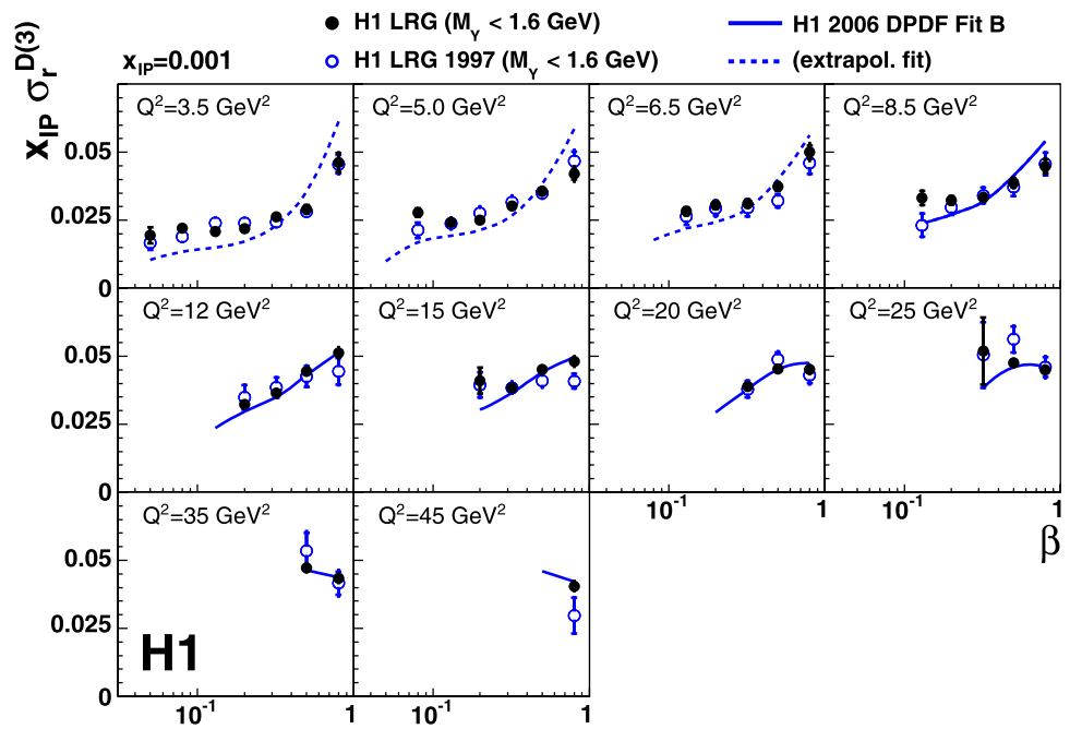
Fig. 4 The \beta dependence of the reduced diffractive cross section, multiplied by x_{\mathbb{P}} , at a fixed value of x_{\mathbb{P}} = 0.001 , resulting from the combination of all data samples. Details are explained in the caption of Fig. 3
