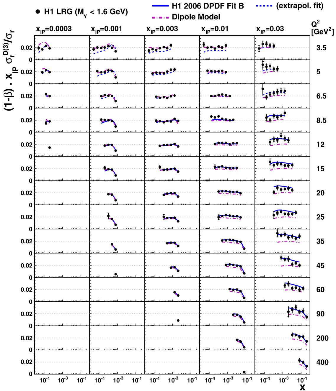
Fig. 11 The ratio of the diffractive to the inclusive reduced cross section, multiplied by (1 - \beta)x_{\mathbb{P}} . The inner and outer error bars on the data points represent the statistical and total uncertainties, respectively.
