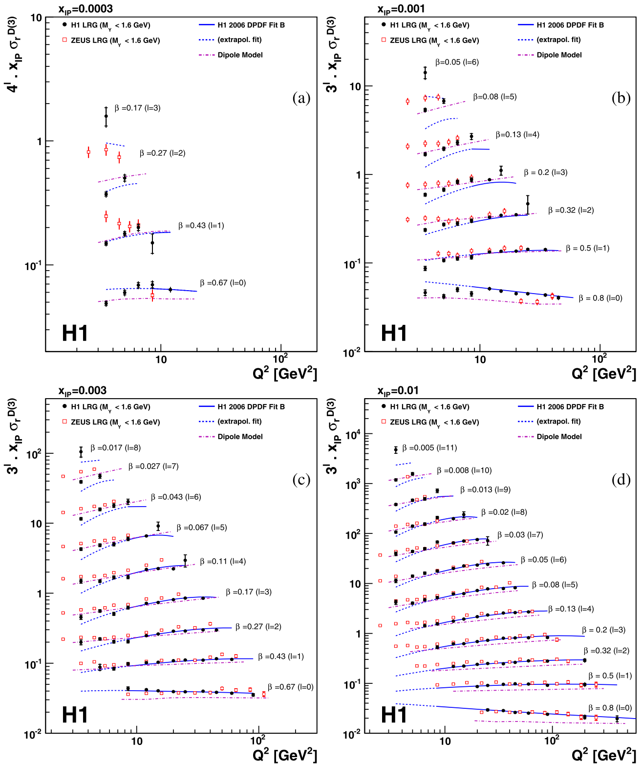
Fig. 10 The Q^2 dependence of the reduced diffractive cross section from combined H1 data, multiplied by x_{IP} , at different fixed values of x_{IP} = 0.0003 (a), 0.001 (b), 0.003 (c) and 0.01 (d). The present data are compared with the results of the ZEUS Collaboration [14], corrected to M_Y < 1.6 GeV (see text). The 8 % overall uncertainty on this
