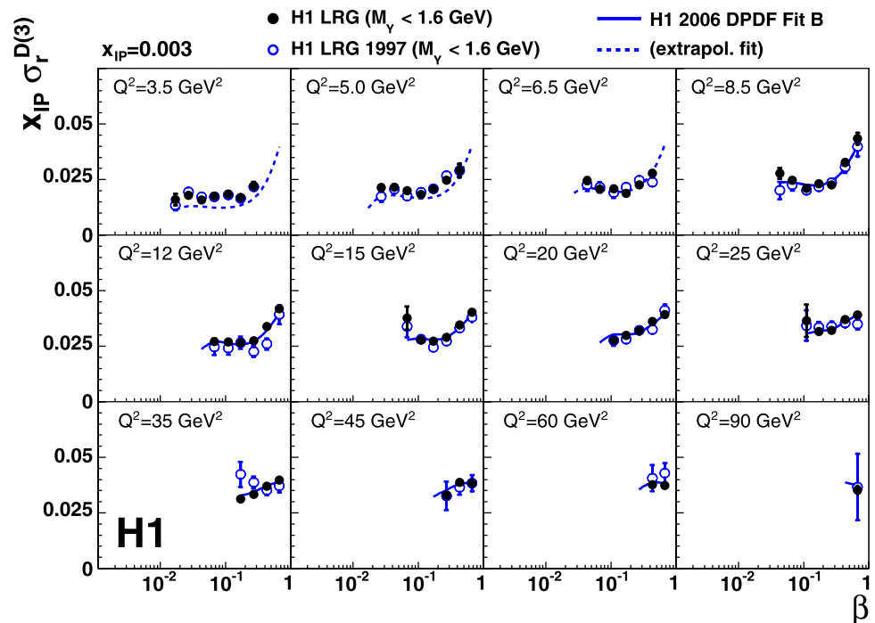
Fig. 5 The \beta dependence of the reduced diffractive cross section, multiplied by x_{\mathbb{P}} , at a fixed value of x_{\mathbb{P}} = 0.003 , resulting from the combination of all data samples. Details are explained in the caption of Fig. 3
