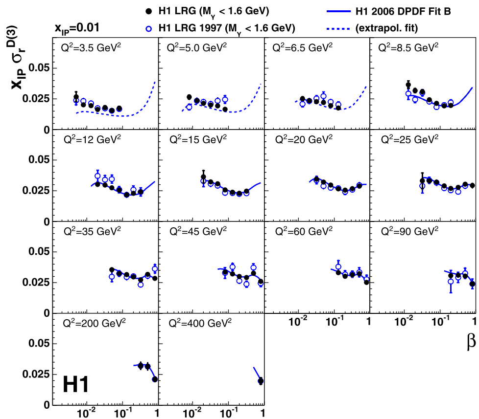
Fig. 6 The \beta dependence of the reduced diffractive cross section, multiplied by x_{\mathbb{P}} , at a fixed value of x_{\mathbb{P}} = 0.01 , resulting from the combination of all data samples. Details are explained in the caption of Fig. 3
