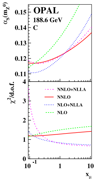
Fig. 7 Results for \alpha_S and \chi^2/\text{d.o.f.} for fits of QCD predictions to the C distribution, as a function of x_\mu
