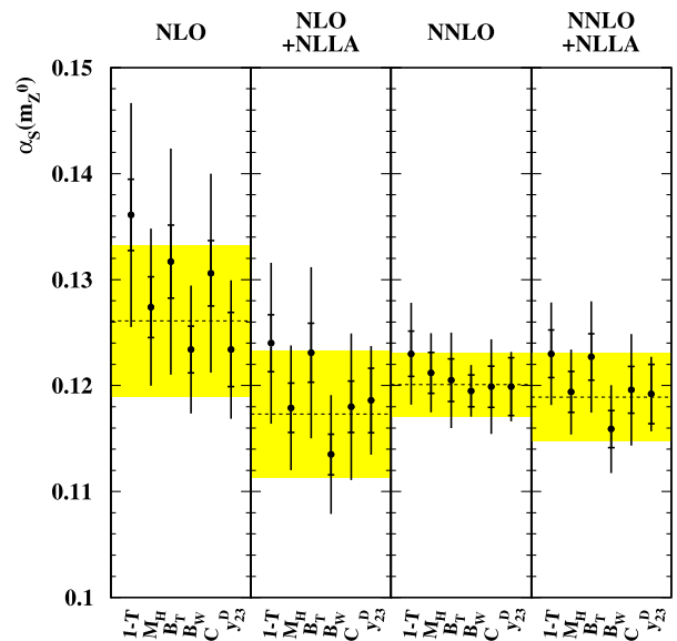
Fig. 6 \alpha_S results combined over all OPAL c.m. energies for different event shape variables and different QCD calculations as indicated on the figure. The shaded bands and dashed lines show the values of \alpha_S(m_{Z^0}) combined from these values with total uncertainties. The inner and outer uncertainty bars show the combined statistical and experimental and total uncertainties, respectively
