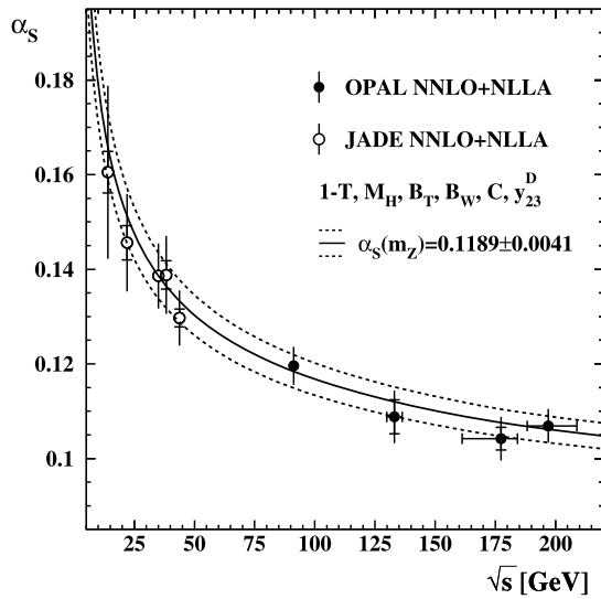
Fig. 5 The points in the above plot show the values of \alpha_S for the OPAL energy ranges which are indicated by the horizontal error bars. The inner uncertainty bars show the combined statistical and experimental uncertainties and the outer the total uncertainties. The full and dashed lines indicate the \alpha_S result from the NNLO + NLLA analysis that combines all variables and OPAL energy points. The results from the NNLO + NLLA analysis of JADE data [12] are shown as well
