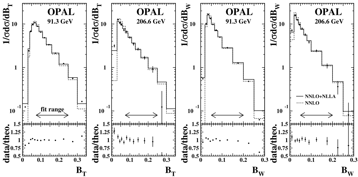
Fig. 3 The points in the upper plots show the B_T and B_W distributions at the hadron level for \sqrt{s} = 91.3 and 206.6 GeV with statistical uncertainty bars. Some uncertainty bars are smaller than the data points. Superimposed as histograms are the NNLO and NNLO + NLLA pre-
