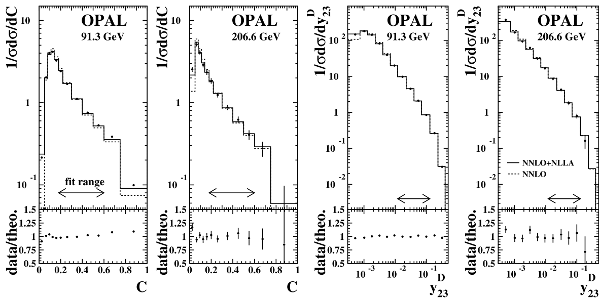
Fig. 4 The points in the upper plots show the C and y_{23}^D distributions at the hadron level for \sqrt{s} = 91.3 and 206.6 GeV with statistical uncertainty bars. Some uncertainty bars are smaller than the data points. Superimposed as histograms are the NNLO and NNLO + NLLA pre-
