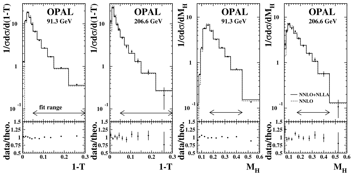
Fig. 2 The points in the upper plots show the 1 - T and M_H distributions at the hadron level for \sqrt{s} = 91.3 and 206.6 GeV with statistical uncertainty bars. Some uncertainty bars are smaller than the data points. Superimposed as histograms are the NNLO and
