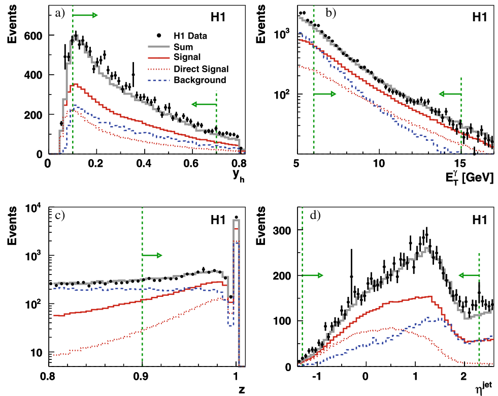
Fig. 2 Distributions of (a) the inelasticity y_h , (b) the transverse energy E_T^y of the photon, (c) the isolation parameter z and (d) \eta^{\text{jet}} for events with prompt photon candidates. Data are shown as points with error bars indicating the statistical error. The signal prediction from PYTHIA for prompt photons is shown as dark full line , and the contribution of direct interactions as a dotted line . The background as simulated with PYTHIA is shown as a dashed line . The signal and background contributions are scaled on average by a factor 1.5 and 1.7, respectively. The sum of the scaled signal and background is shown as the light gray histogram . The vertical dashed lines indicate the kinematic region of the cross section measurement
